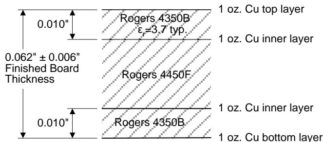
Qorvo PCB 290375 Material and Stack-up
